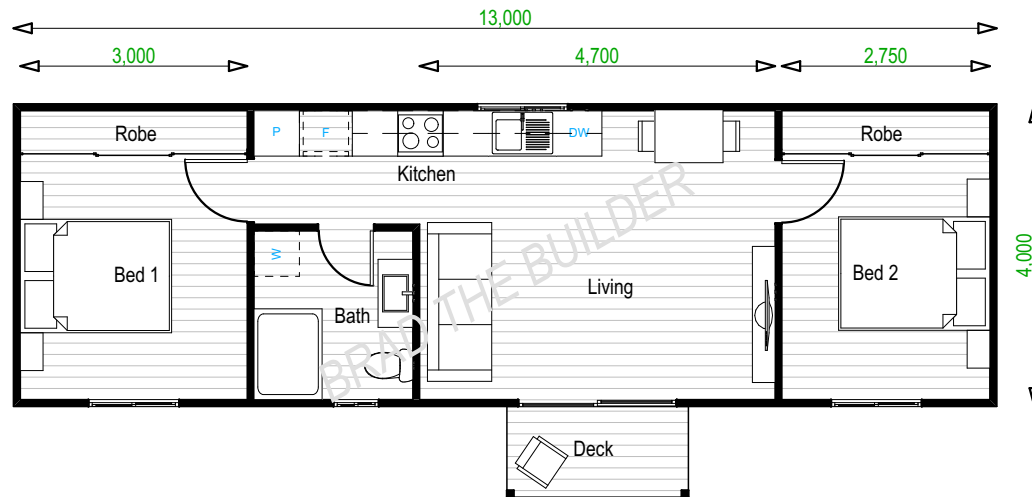
WOODSMAN 52 2x1 - perfect for your 15m wide block
